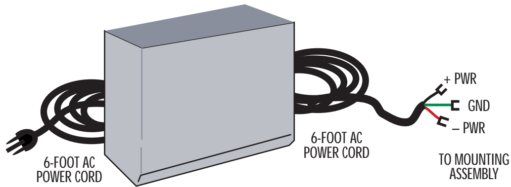
2100-0300 Wiring Diagram
